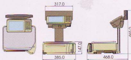
SM-5500EV (Elevated)
