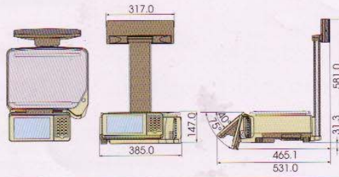
SM-5500EV (Elevated)
